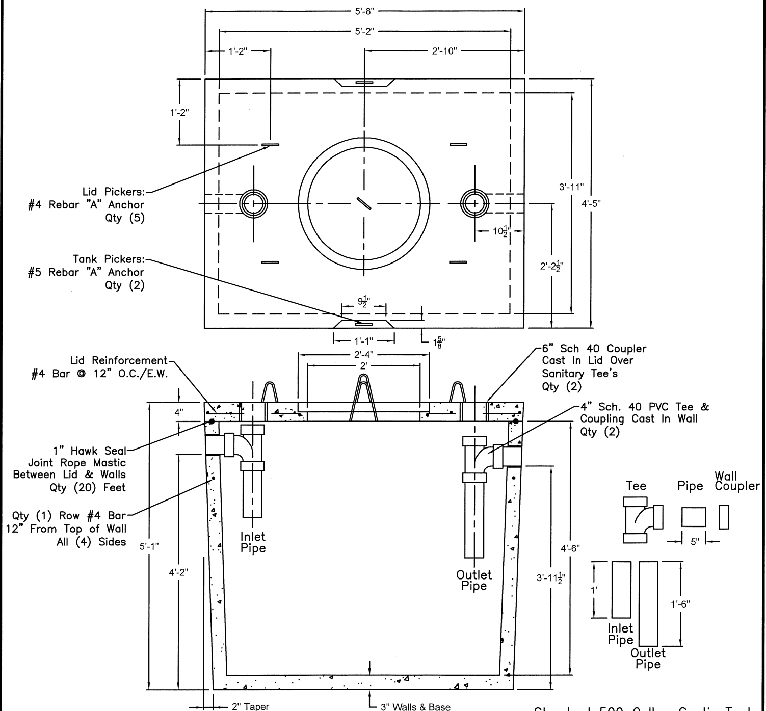
Standard 500 Gallon Septic Tank
